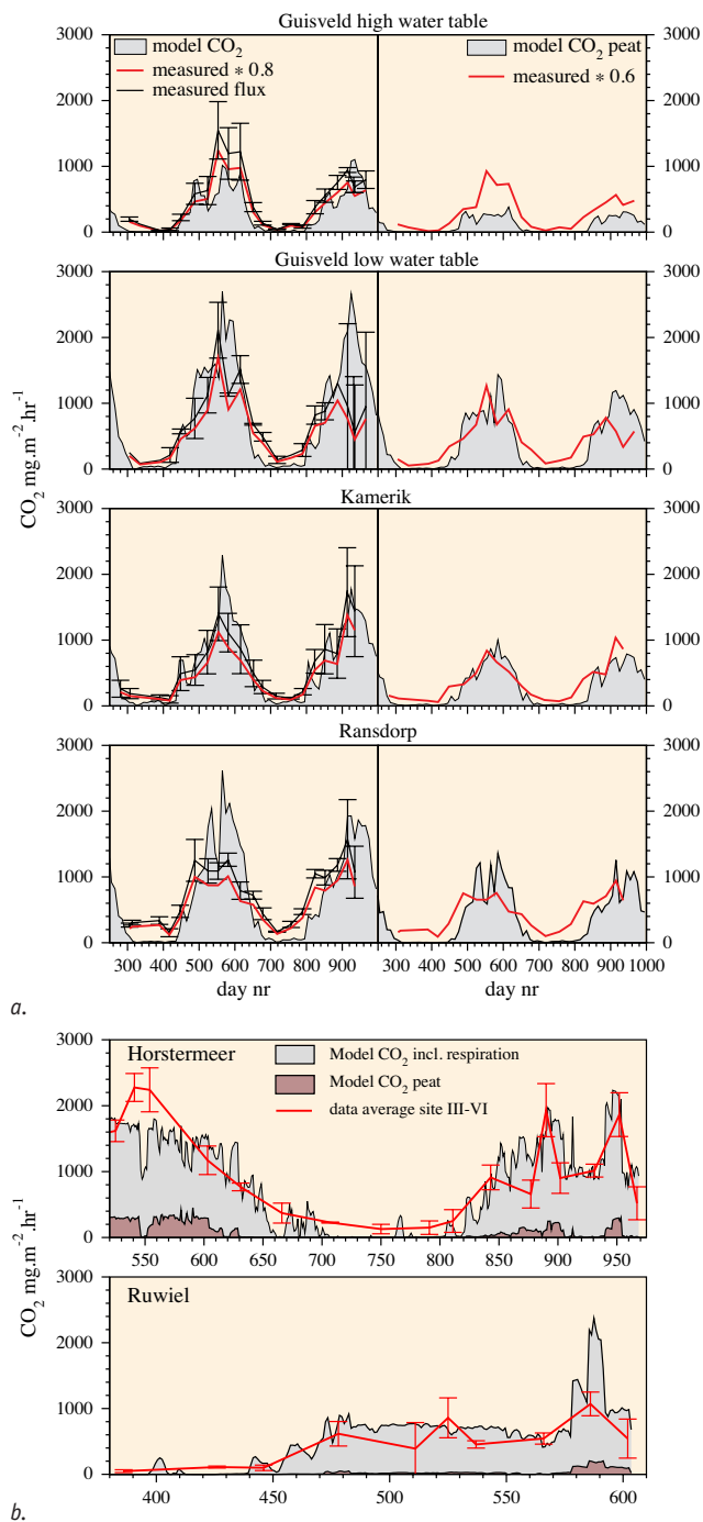
Fig. 4. Comparison of measurement data and model results for all sites for the \text{CO}_2 fluxes. The error bars represent standard deviations of between-station averaged flux measurements. Reference date for the x-axis is January 1, 1998. The left side graphs for the Guisveld, Kamerik and Ransdorp site compare the total model flux (without plant respiration) with the measured fluxes multiplied by a factor of 0.8 to correct for dark respiration of plants during the measurements. The right side graphs compare the modelled flux from the peat reservoir with the measured fluxes multiplied by 0.6 cf. Van den Bos & Van de Plassche (2003a,b). For the Horstermeer and Ruwiel sites, the \text{CO}_2 flux has been compared with the simulated soil \text{CO}_2 flux plus a modelled estimate of dark respiration of the plants. Reference dates for the time axis are resp. January 1, 2002 and January 1, 2003, model time step is 1 day.
