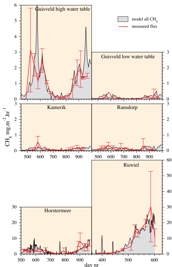
Fig. 5. Measured \text{CH}_4 fluxes compared with modelled fluxes (total flux, including diffusion, ebullition and plant fluxes) for all sites. Model time step and reference dates for time axes as in Fig. 4.
