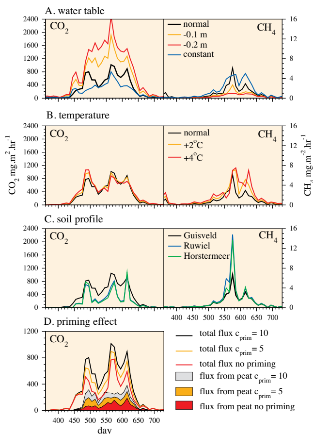
Fig. 6. Sensitivity test results. Modelled flux time series over one year are shown. The sensitivity tests are based on the temperature and water table time series and soil profile at the Guisveld site; the model run indicated as 'normal' represents the validation model run for Guisveld high water table in Fig. 4. Note different scale for the latter graph.
